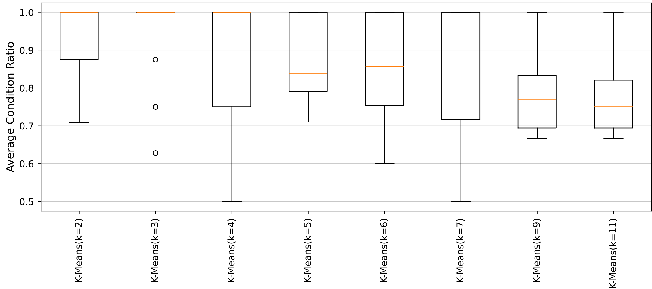
YARA Rules Average Condition Ratio Distribution (Cluster9_Size11 dataset)
